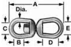
Galvanized Forged Steel Eye and Eye
