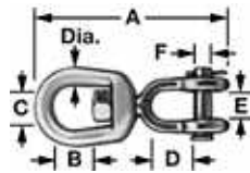
Eye and Fork with Cotter Pin
