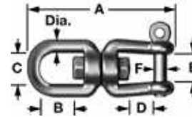
Eye and Fork with Screw Pin
