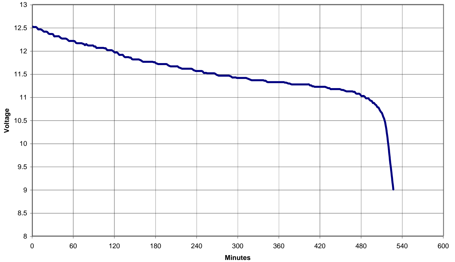
11.1 Volts 800 mAh (15C) Li-Ion/Poly 100 mA discharge
